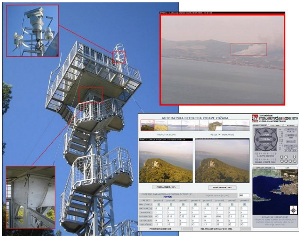
Figure 1. Croatian iForestFire monitoring station in experimental work on Marjan hill (Split area) during 2005 and 2006 fire season
